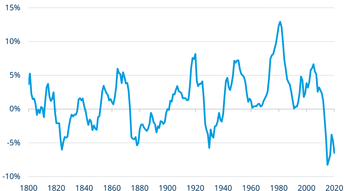
Figure 3. Commodity supercycles (1800–2020)
